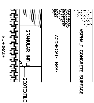
PAVEMENT SUBBASE STABILIZATION
